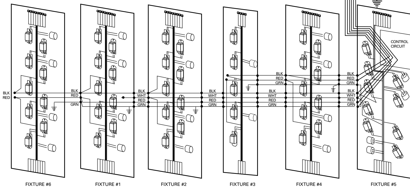
60 HZ 3/1 PHASE SYSTEM SCHEMATIC
