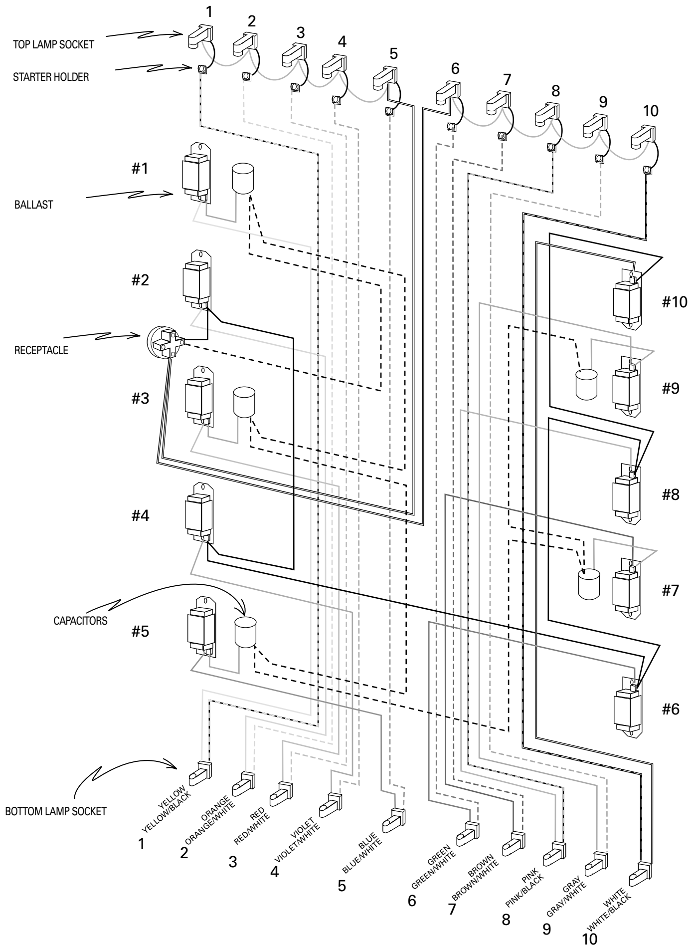
10 LAMP FIXTURE WIRING
