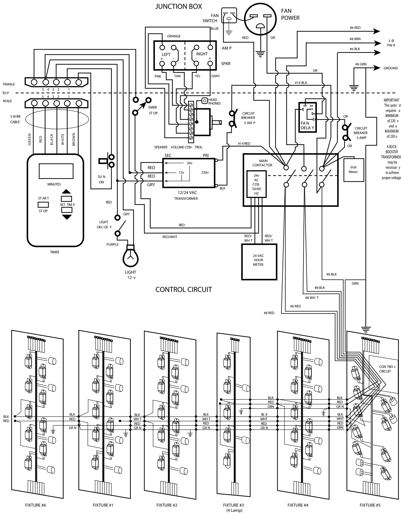
60 HZ 3/1 PHASE SYSTEM SCHEMATIC
