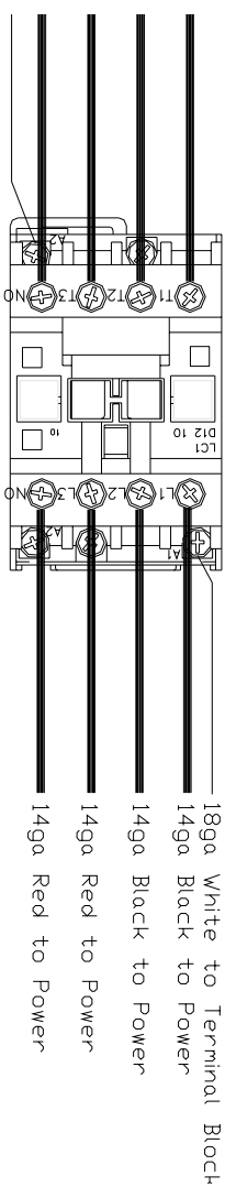
Relay Panel C
